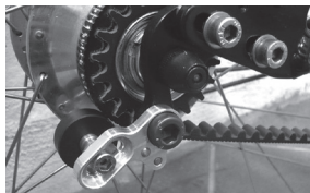
Illustration 1: Rohloff SPEEDHUB 500/14 with Snubber
