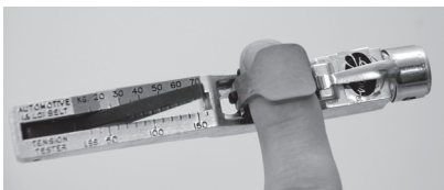
Securing the Tension Tester (Art. No 10400009)
